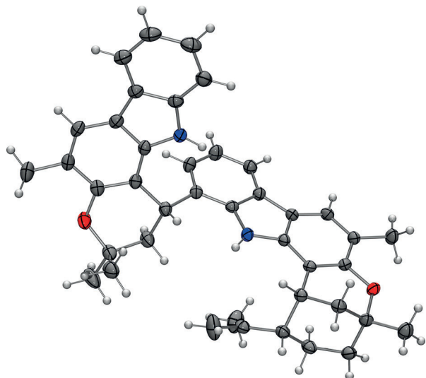
Figure 1. Molecular structure of murrufoline A ( 1 ) in the crystal (ORTEP plot showing thermal ellipsoids at the 50% probability level).
